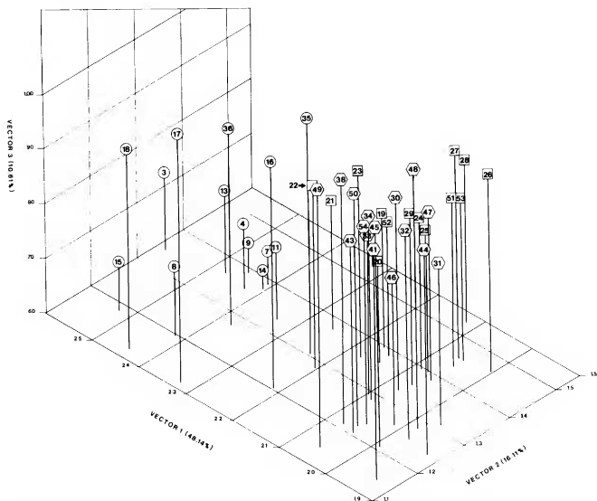
FIG. 13.—Three-dimensional projections of the 44 samples of Geomys burbarius females onto the first three canonical vectors. Circles represent the lutescens chromosome group; squares, the attwateri group; and hexagons, the breviceps group.
